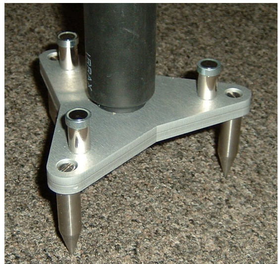
Sensor HU 9 with support
